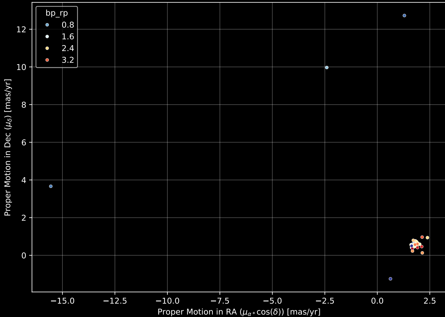
APOGEE DR17 Field: [280-32-O] Proper Motion Diagram (n= 39)
