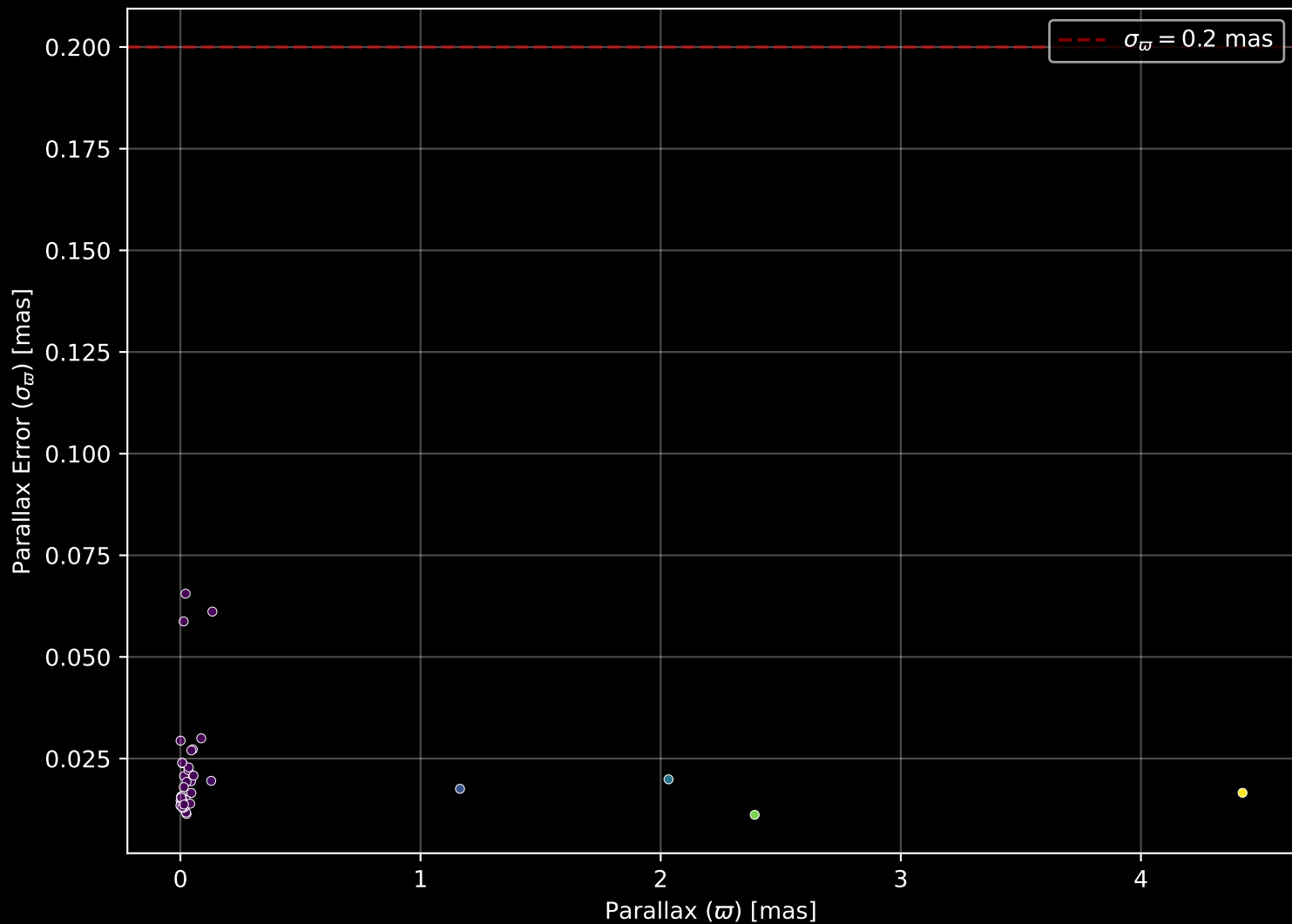
APOGEE DR17 Field: [280-32-O] Parallax Quality (n= 39)
