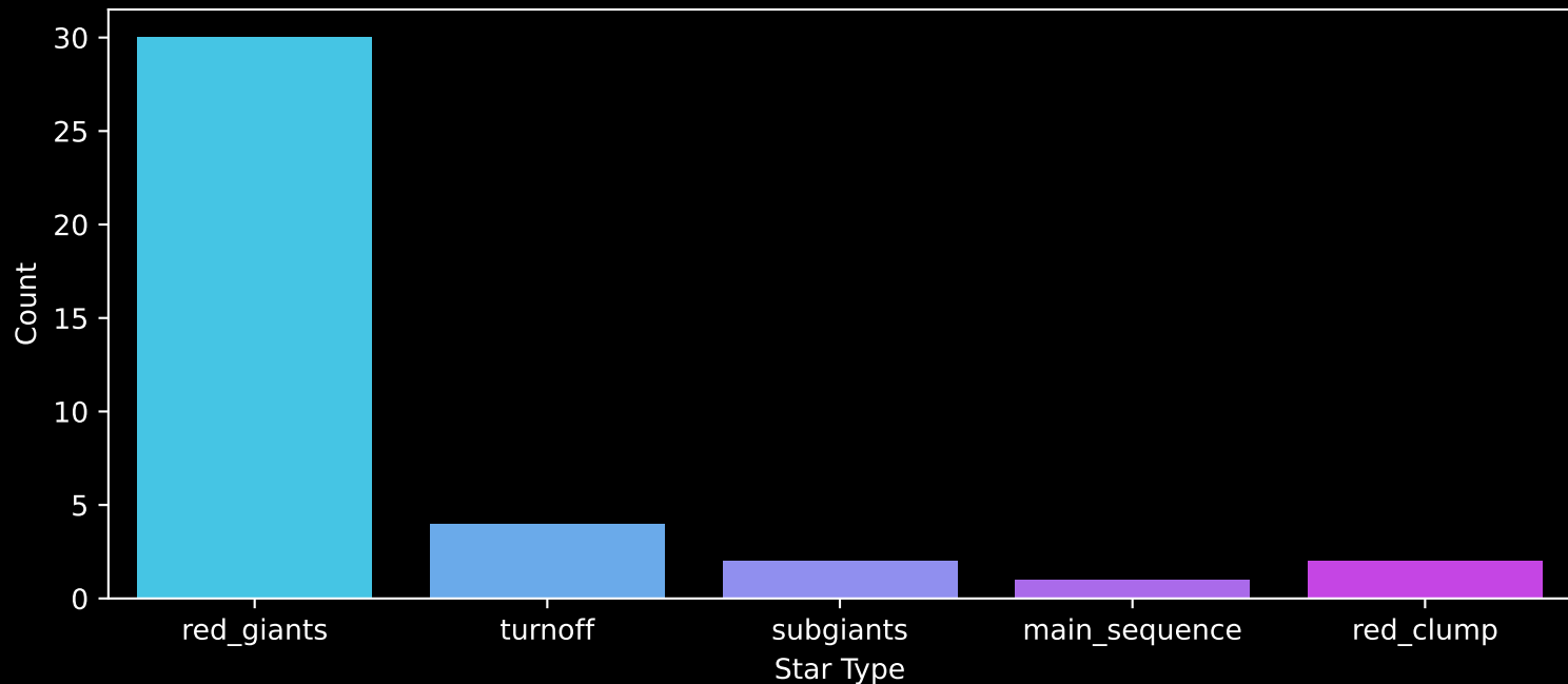
APOGEE DR17 Field: [280-32-O] Count plot of Star Type
