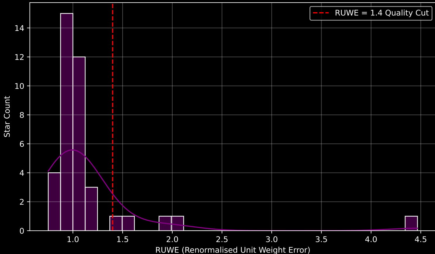
GAPOGEE DR17 Field [280-32-O] RUWE Distribution (n= 39)
